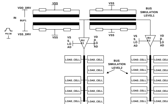
CLOCK TREE EXAMPLE USING 2 LEVEL HIERARCHICAL BUS
